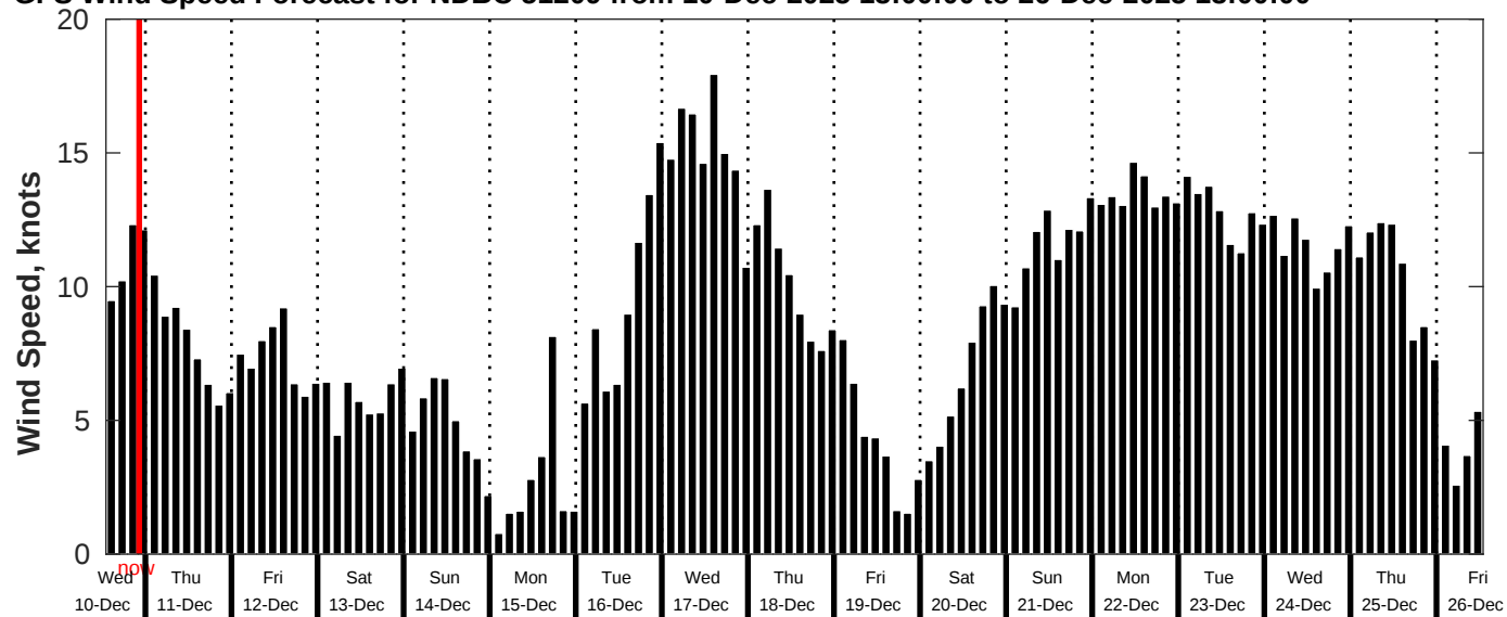
GFS Wind Speed Forecast for NDBC 51209 from 10-Dec-2025 13:00:00 to 26-Dec-2025 13:00:00
