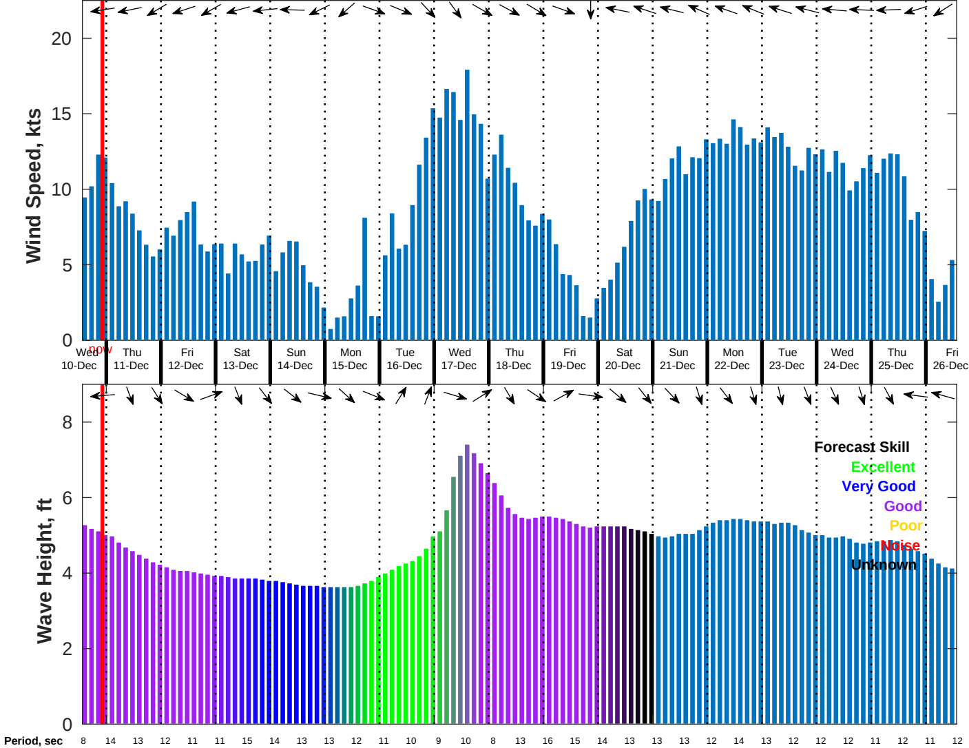
Wind & Wave Forecast for NDBC 51209 from 10-Dec-2025 13:00:00 to 26-Dec-2025 13:00:00
