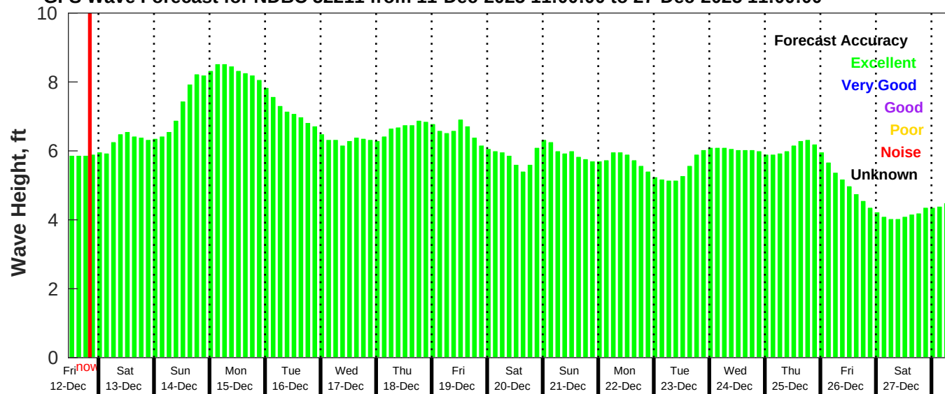
GFS Wave Forecast for NDBC 52211 from 11-Dec-2025 11:00:00 to 27-Dec-2025 11:00:00
