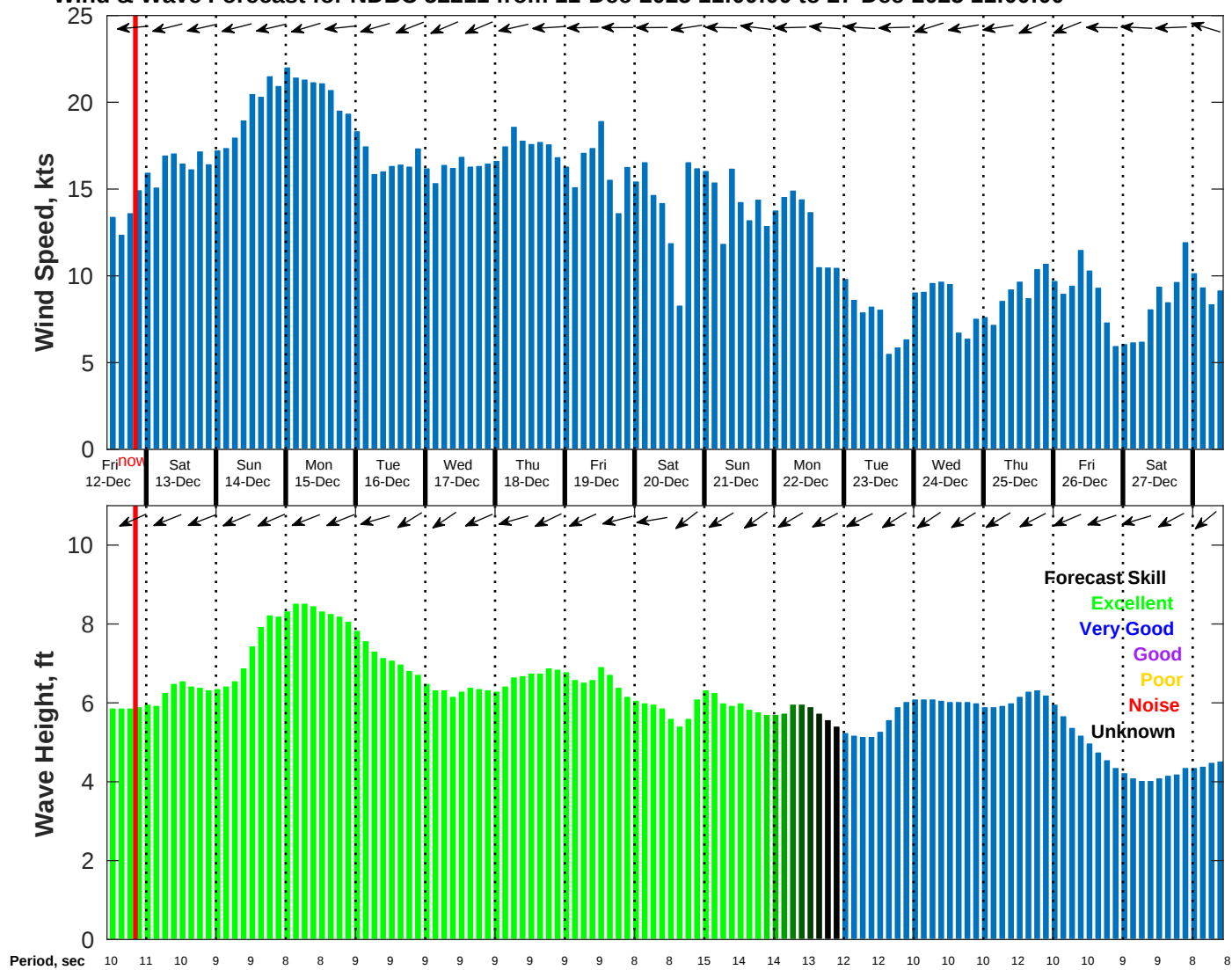
Wind & Wave Forecast for NDBC 52211 from 11-Dec-2025 11:00:00 to 27-Dec-2025 11:00:00
