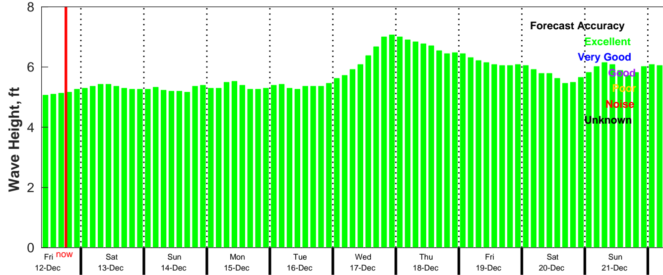
CMEMS Wave Forecast for NDBC 52212 from 11-Dec-2025 09:00:00 to 21-Dec-2025 09:00:00
