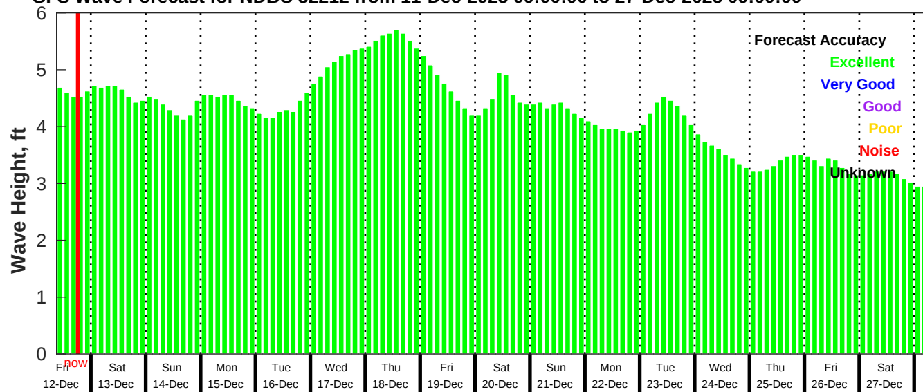
GFS Wave Forecast for NDBC 52212 from 11-Dec-2025 09:00:00 to 27-Dec-2025 09:00:00
