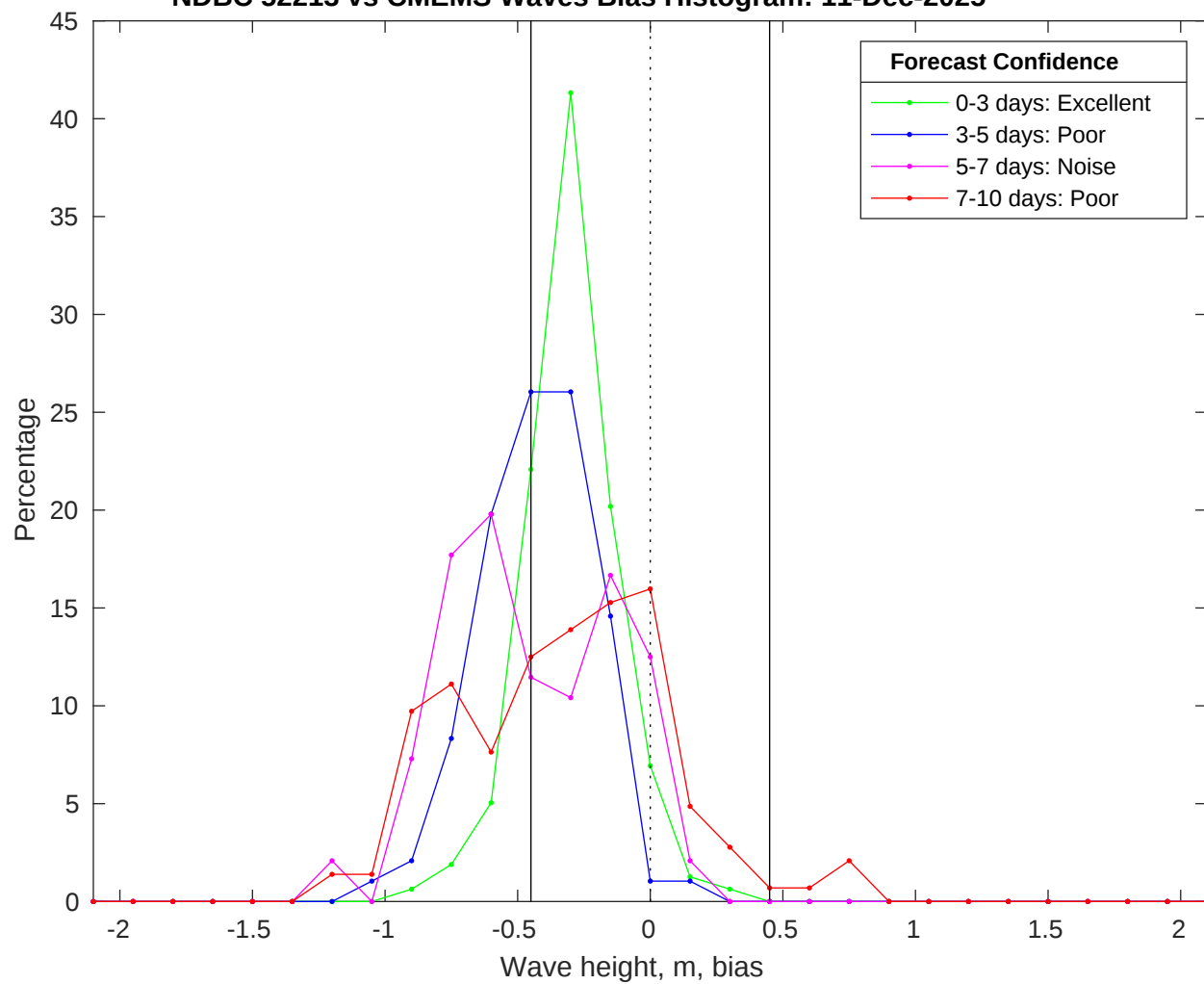
NDBC 52213 vs CMEMS Waves Bias Histogram: 11-Dec-2025
