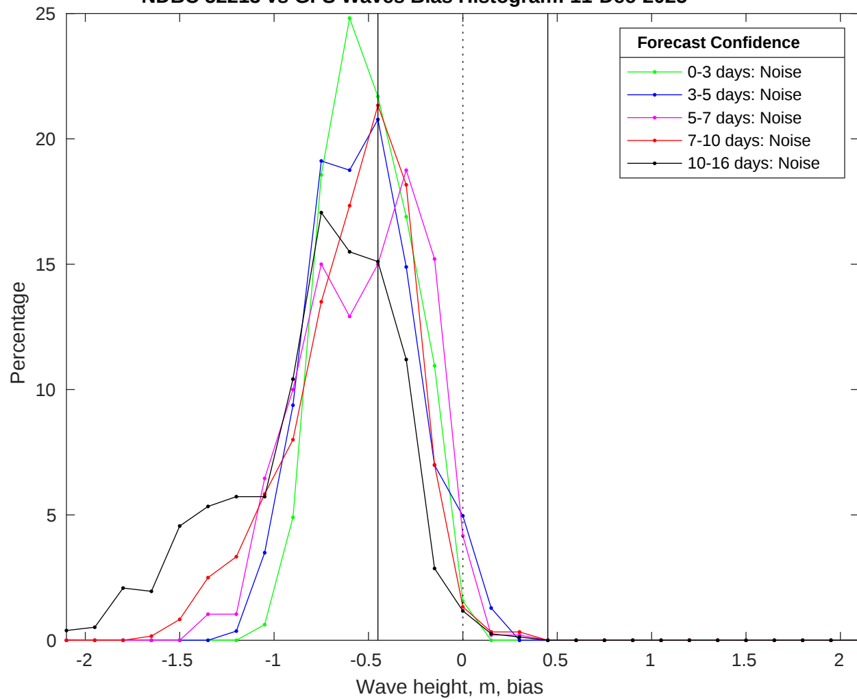
NDBC 52213 vs GFS Waves Bias Histogram: 11-Dec-2025
