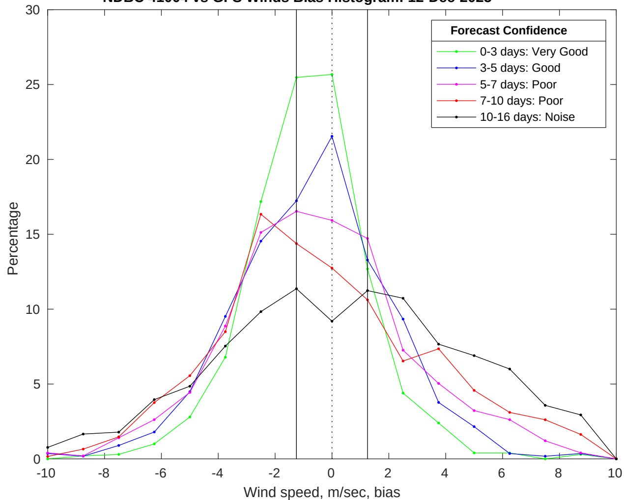
NDBC 41004 vs GFS Winds Bias Histogram: 12-Dec-2025
