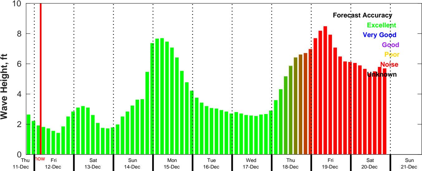
CMEMS Wave Forecast for NDBC 41004 from 11-Dec-2025 19:00:00 to 21-Dec-2025 19:00:00
