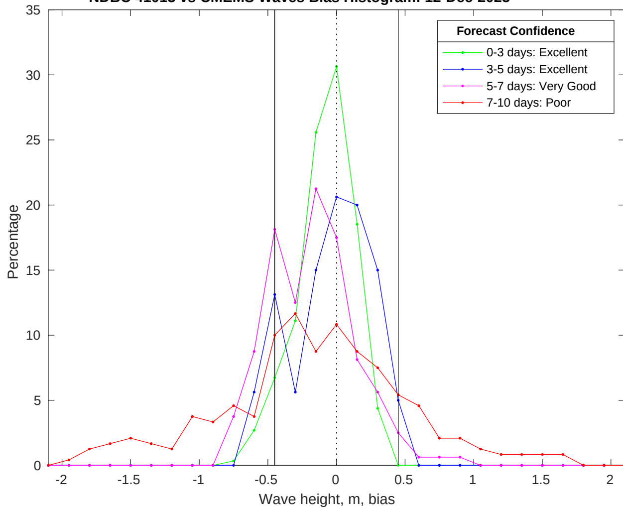
NDBC 41013 vs CMEMS Waves Bias Histogram: 12-Dec-2025
