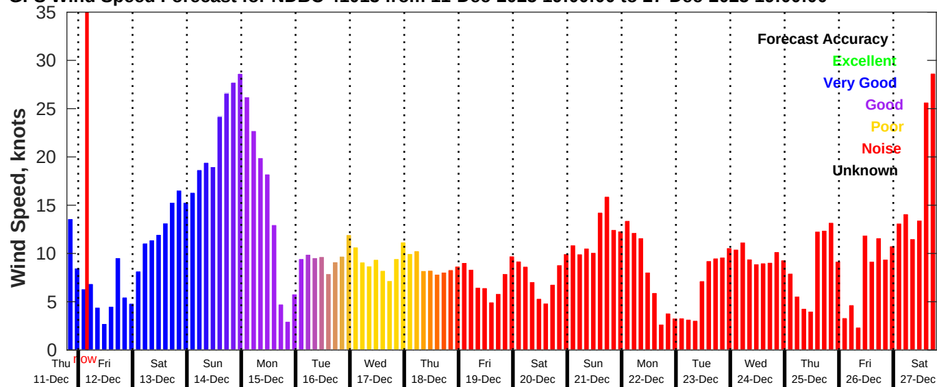
GFS Wind Speed Forecast for NDBC 41013 from 11-Dec-2025 19:00:00 to 27-Dec-2025 19:00:00
