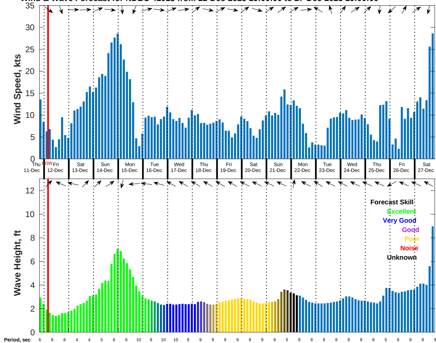
Wind & Wave Forecast for NDBC 41013 from 11-Dec-2025 19:00:00 to 27-Dec-2025 19:00:00
