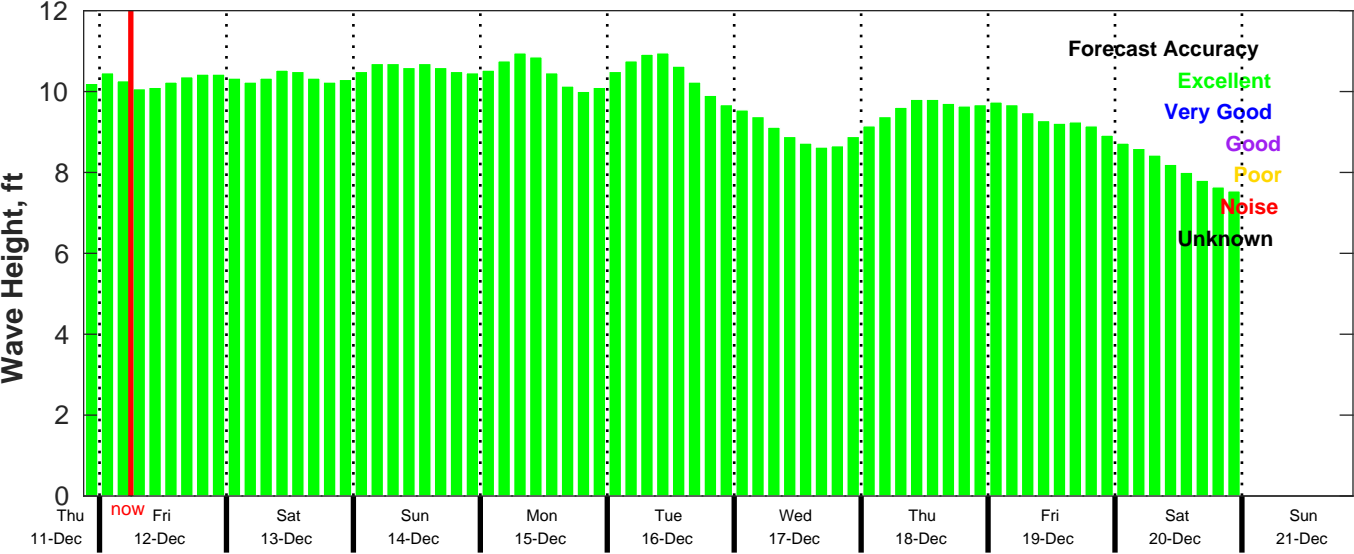
CMEMS Wave Forecast for NDBC 41040 from 11-Dec-2025 21:00:00 to 21-Dec-2025 21:00:00
