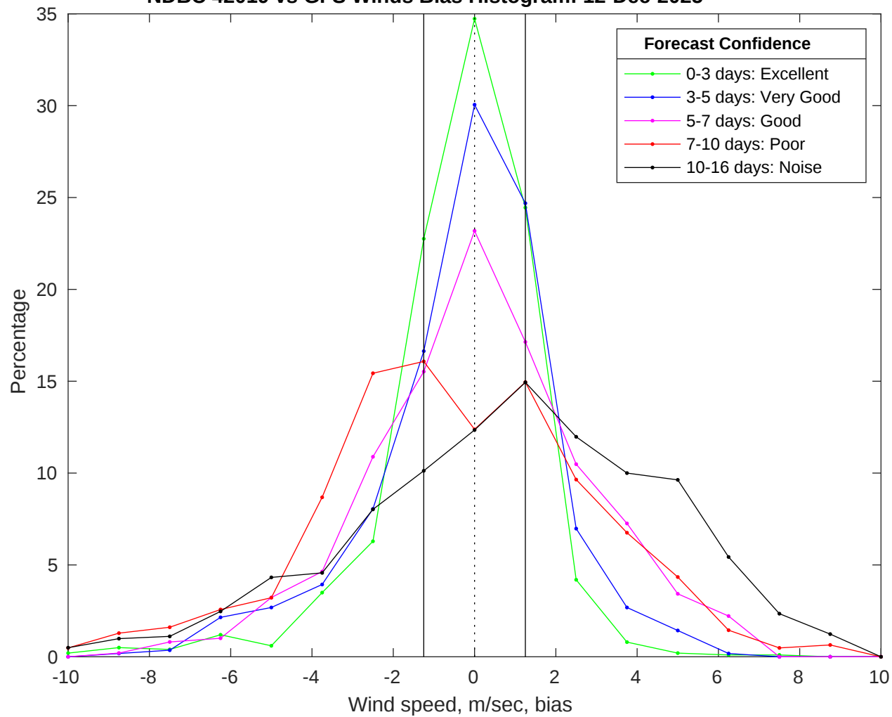
NDBC 42019 vs GFS Winds Bias Histogram: 12-Dec-2025
