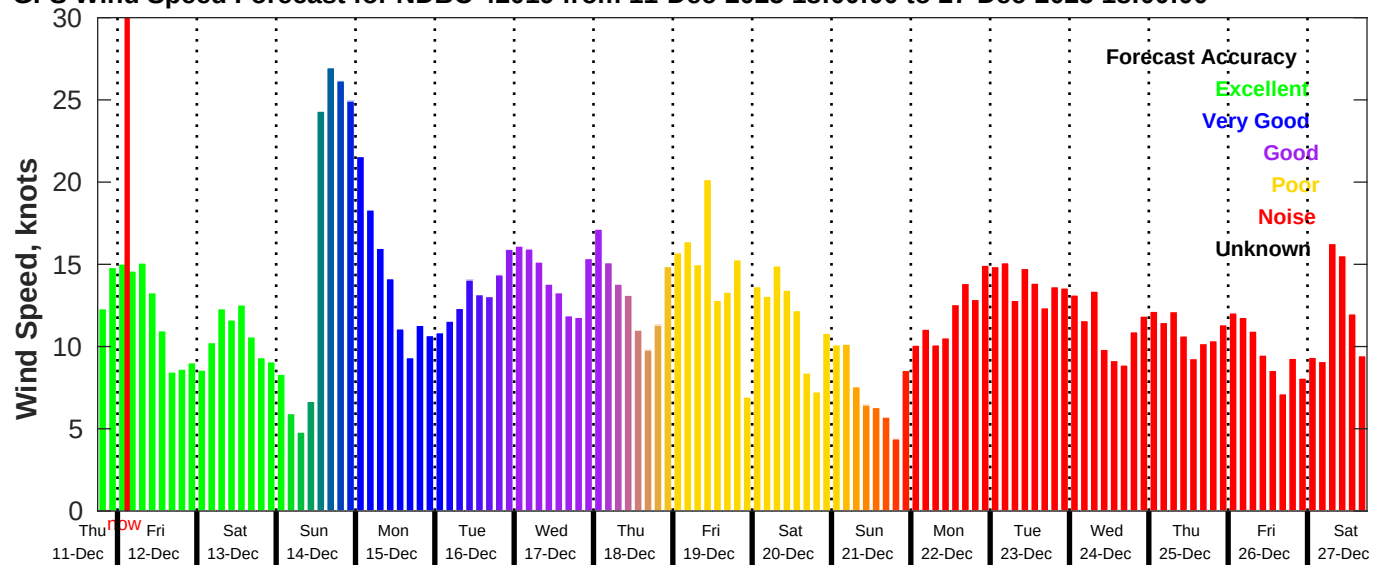
GFS Wind Speed Forecast for NDBC 42019 from 11-Dec-2025 18:00:00 to 27-Dec-2025 18:00:00
