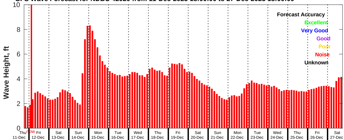
GFS Wave Forecast for NDBC 42020 from 11-Dec-2025 18:00:00 to 27-Dec-2025 18:00:00
