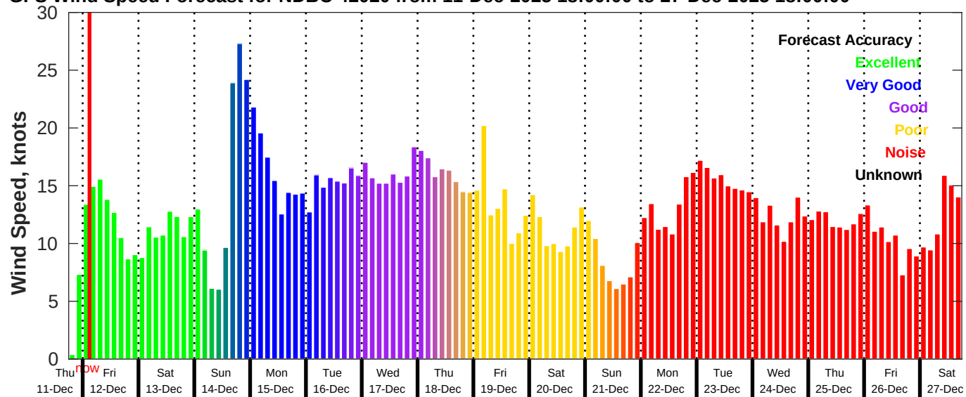
GFS Wind Speed Forecast for NDBC 42020 from 11-Dec-2025 18:00:00 to 27-Dec-2025 18:00:00
