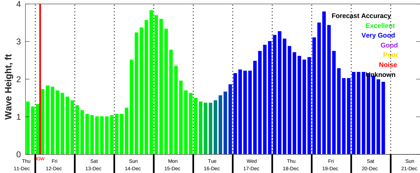
CMEMS Wave Forecast for NDBC 42035 from 11-Dec-2025 18:00:00 to 21-Dec-2025 18:00:00
