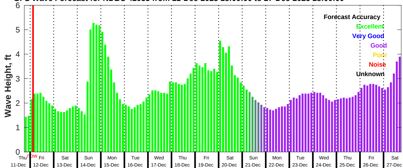
GFS Wave Forecast for NDBC 42035 from 11-Dec-2025 18:00:00 to 27-Dec-2025 18:00:00
