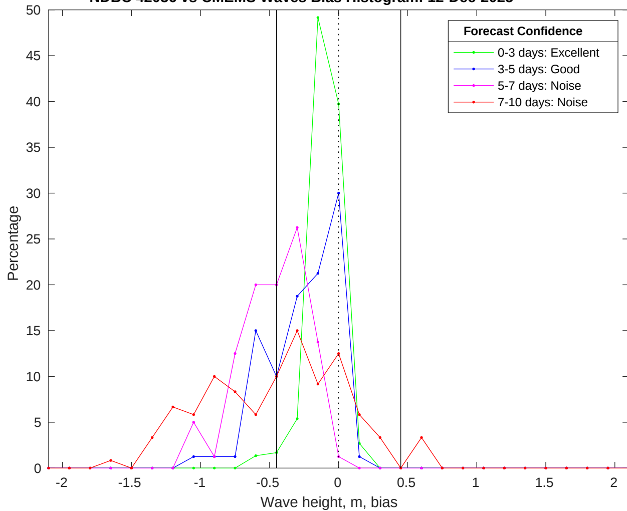
NDBC 42036 vs CMEMS Waves Bias Histogram: 12-Dec-2025
