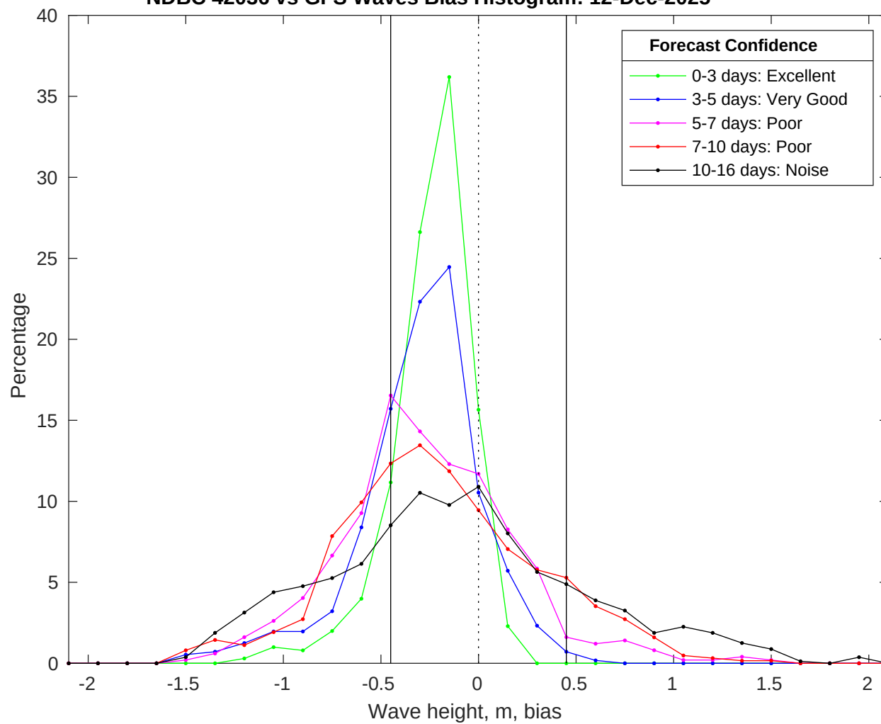
NDBC 42036 vs GFS Waves Bias Histogram: 12-Dec-2025
