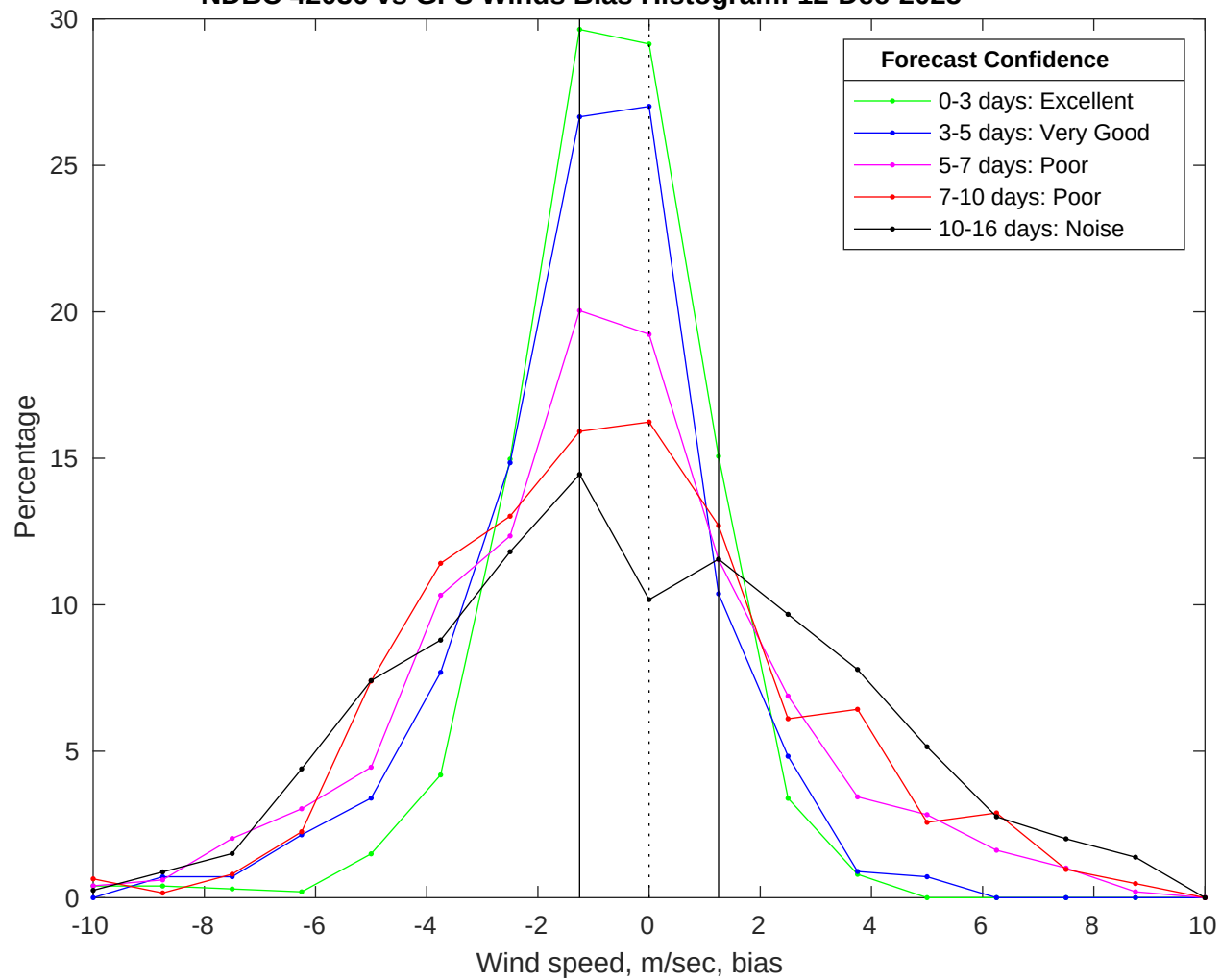
NDBC 42036 vs GFS Winds Bias Histogram: 12-Dec-2025
