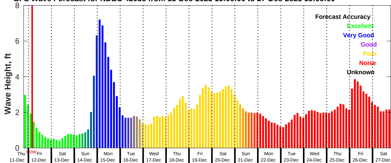
GFS Wave Forecast for NDBC 42036 from 11-Dec-2025 19:00:00 to 27-Dec-2025 19:00:00
