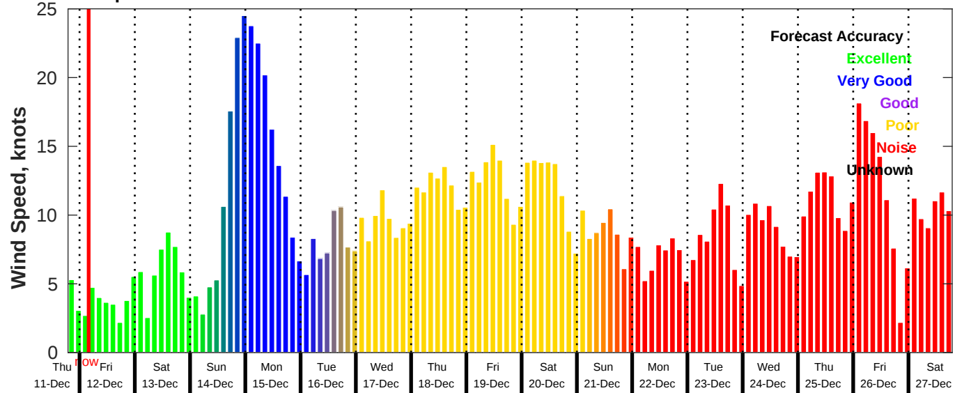
GFS Wind Speed Forecast for NDBC 42036 from 11-Dec-2025 19:00:00 to 27-Dec-2025 19:00:00
