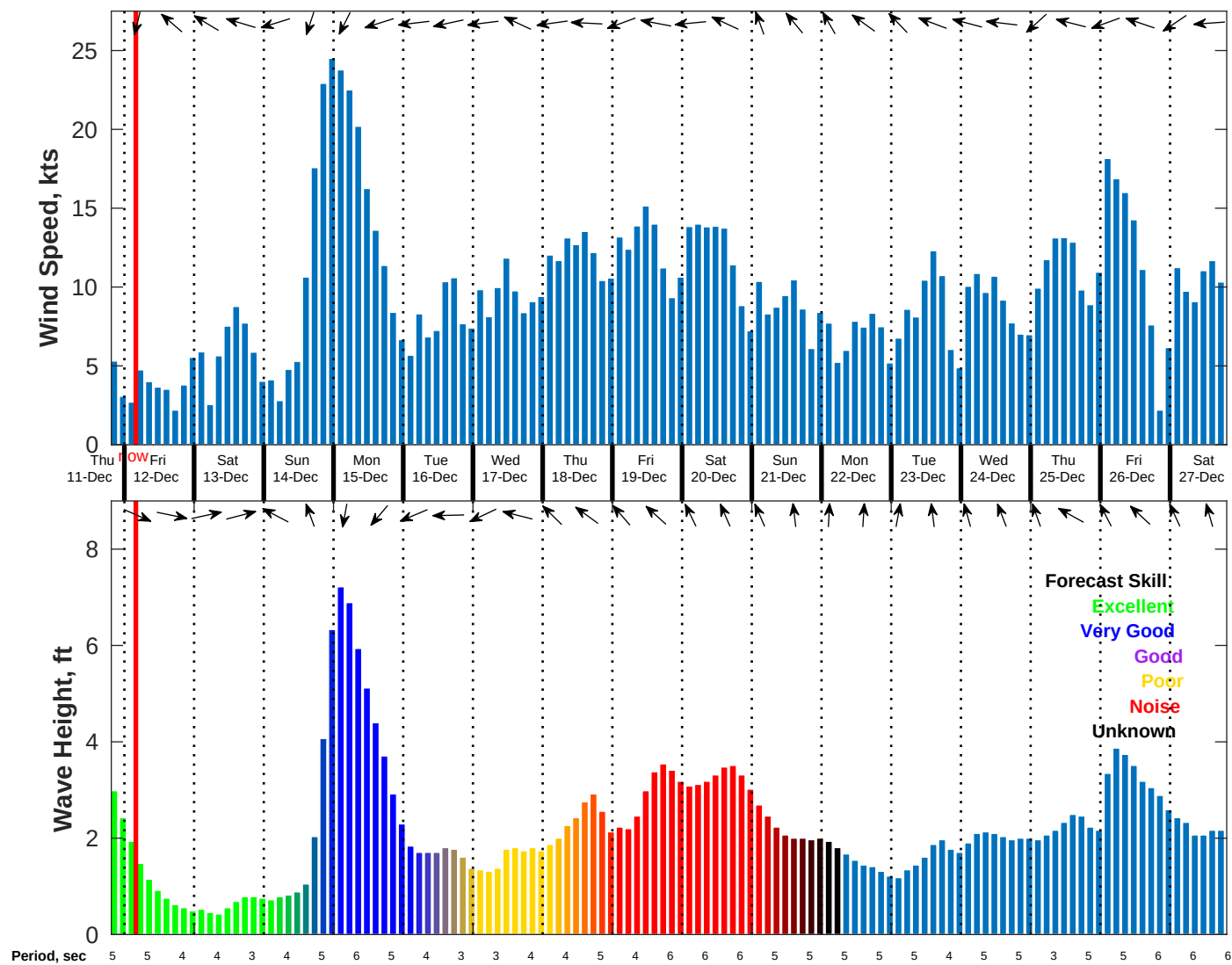
Wind & Wave Forecast for NDBC 42036 from 11-Dec-2025 19:00:00 to 27-Dec-2025 19:00:00
