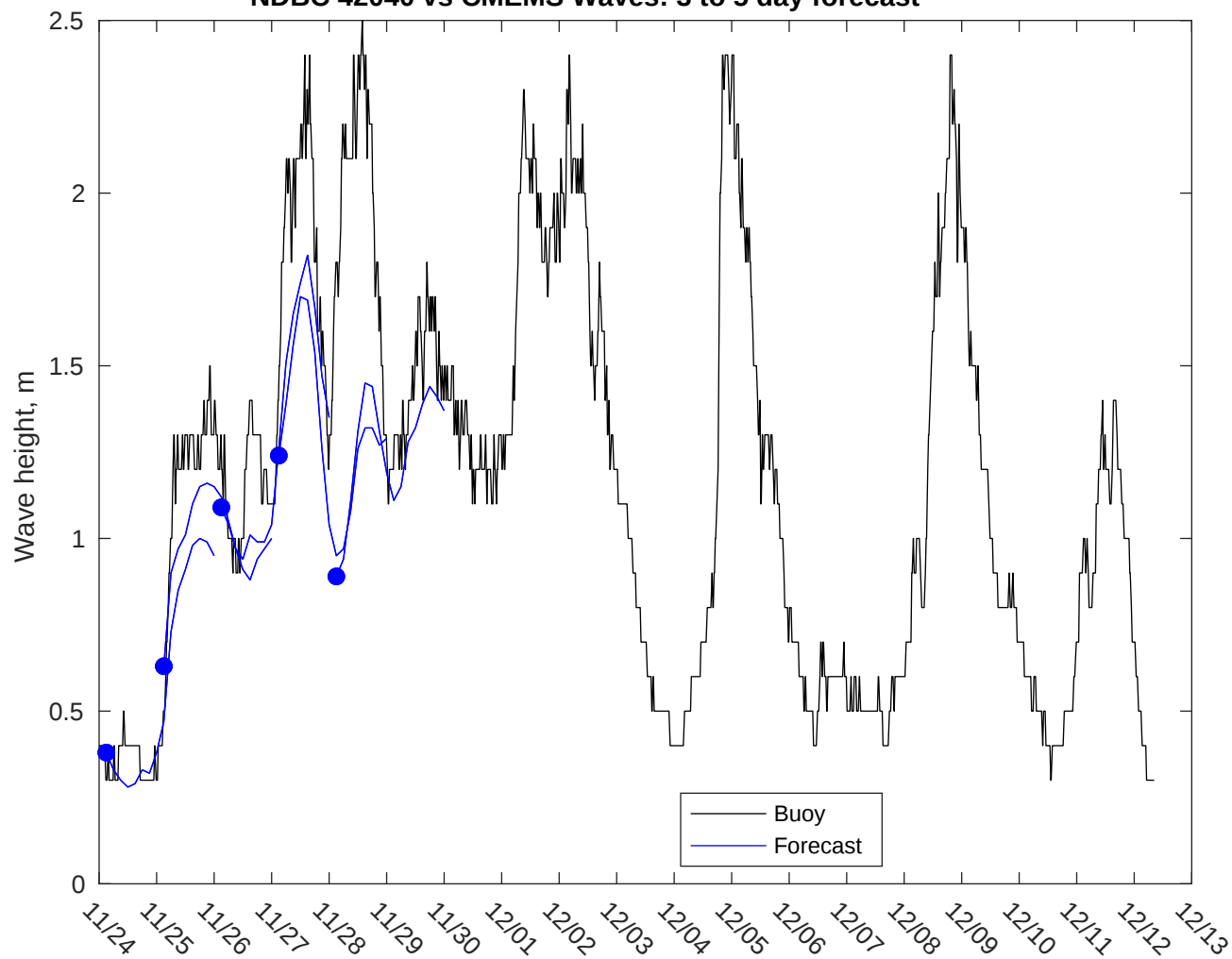
NDBC 42040 vs CMEMS Waves: 3 to 5 day forecast
