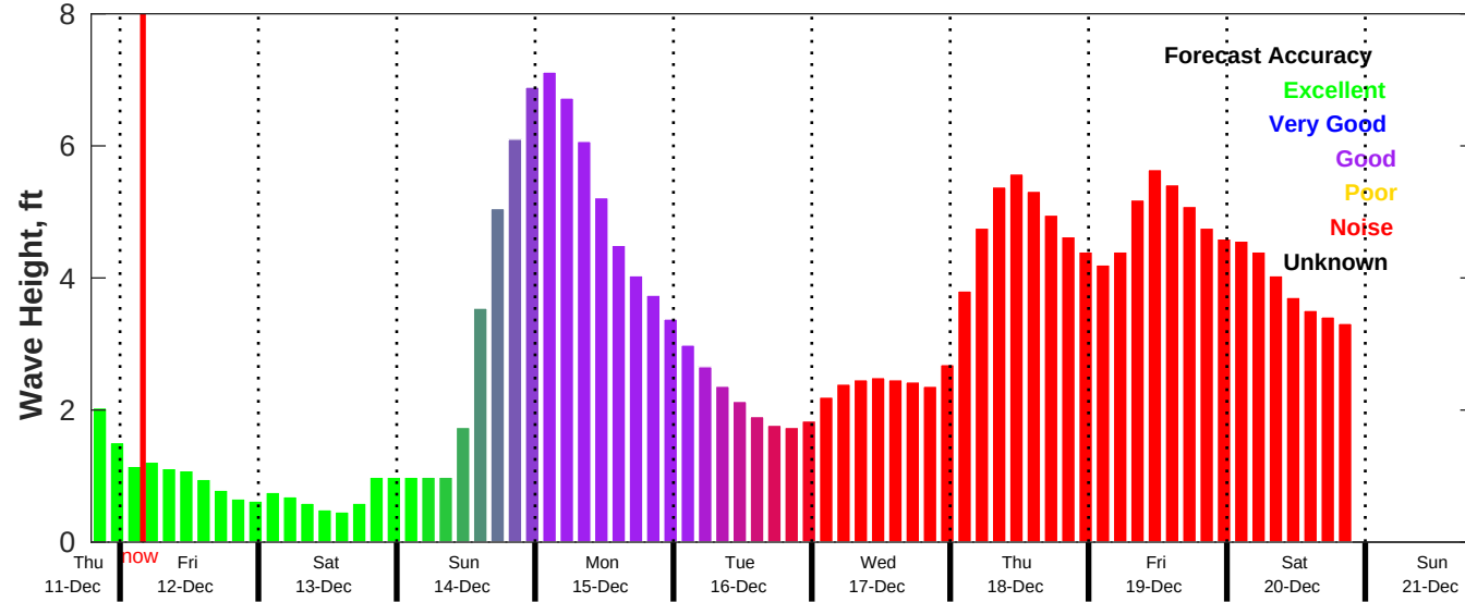
CMEMS Wave Forecast for NDBC 42040 from 11-Dec-2025 19:00:00 to 21-Dec-2025 19:00:00
