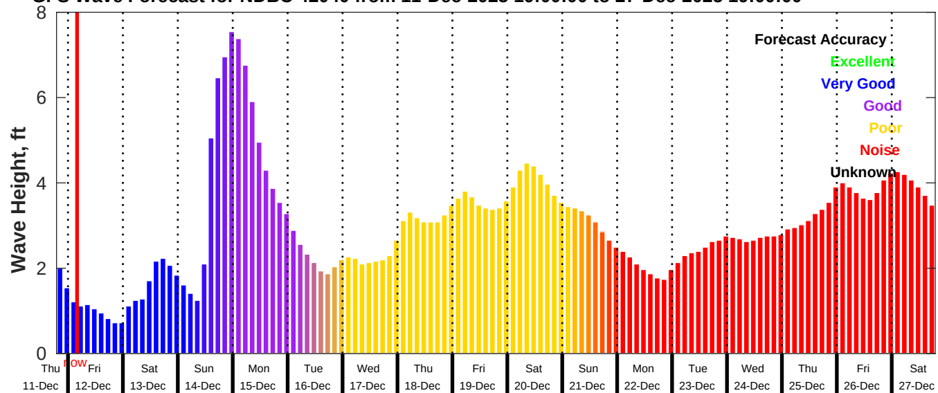
GFS Wave Forecast for NDBC 42040 from 11-Dec-2025 19:00:00 to 27-Dec-2025 19:00:00
