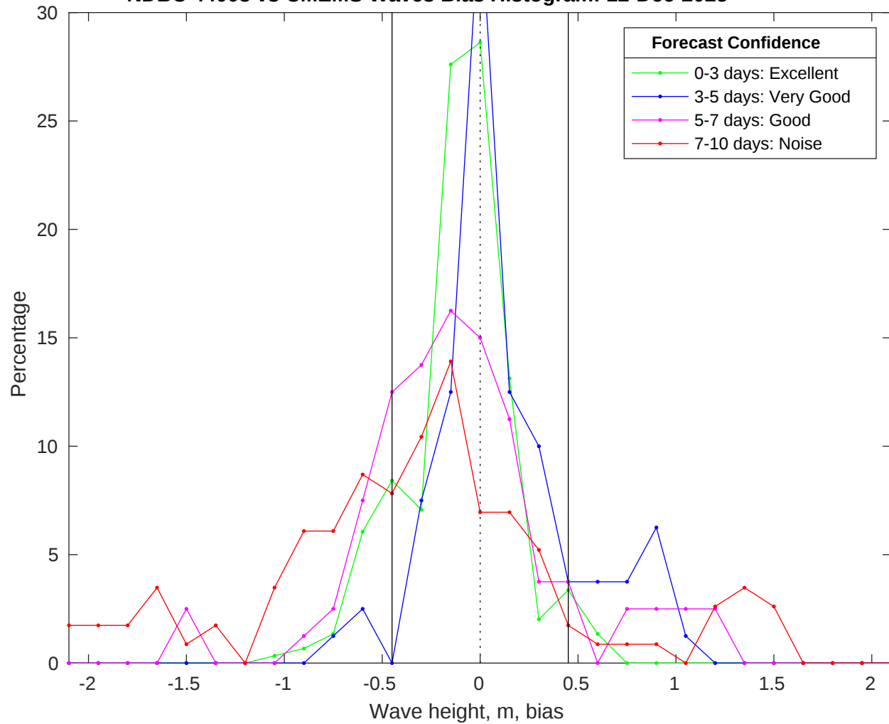
NDBC 44008 vs CMEMS Waves Bias Histogram: 12-Dec-2025
