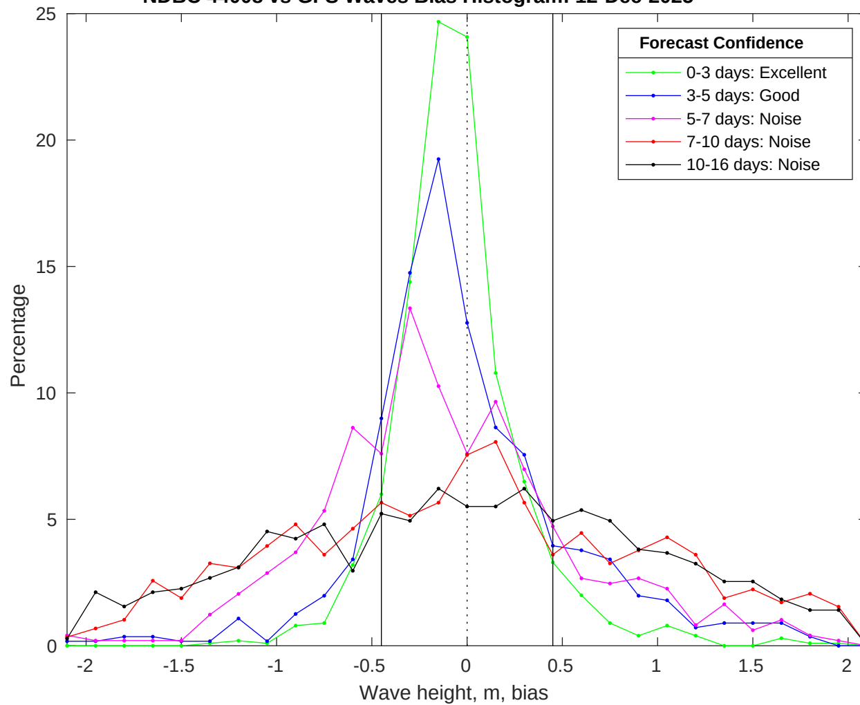
NDBC 44008 vs GFS Waves Bias Histogram: 12-Dec-2025
