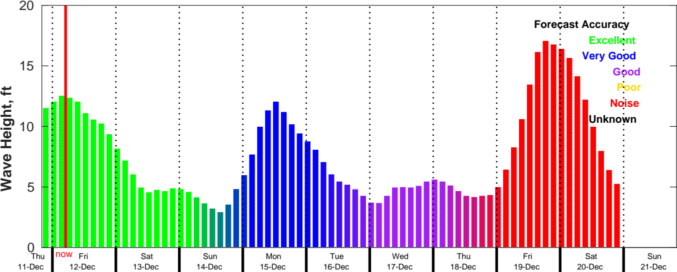
CMEMS Wave Forecast for NDBC 44008 from 11-Dec-2025 20:00:00 to 21-Dec-2025 20:00:00
