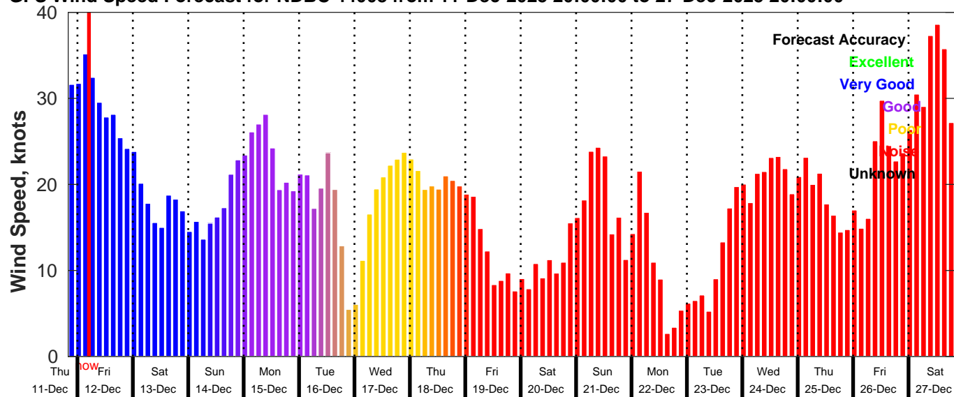
GFS Wind Speed Forecast for NDBC 44008 from 11-Dec-2025 20:00:00 to 27-Dec-2025 20:00:00
