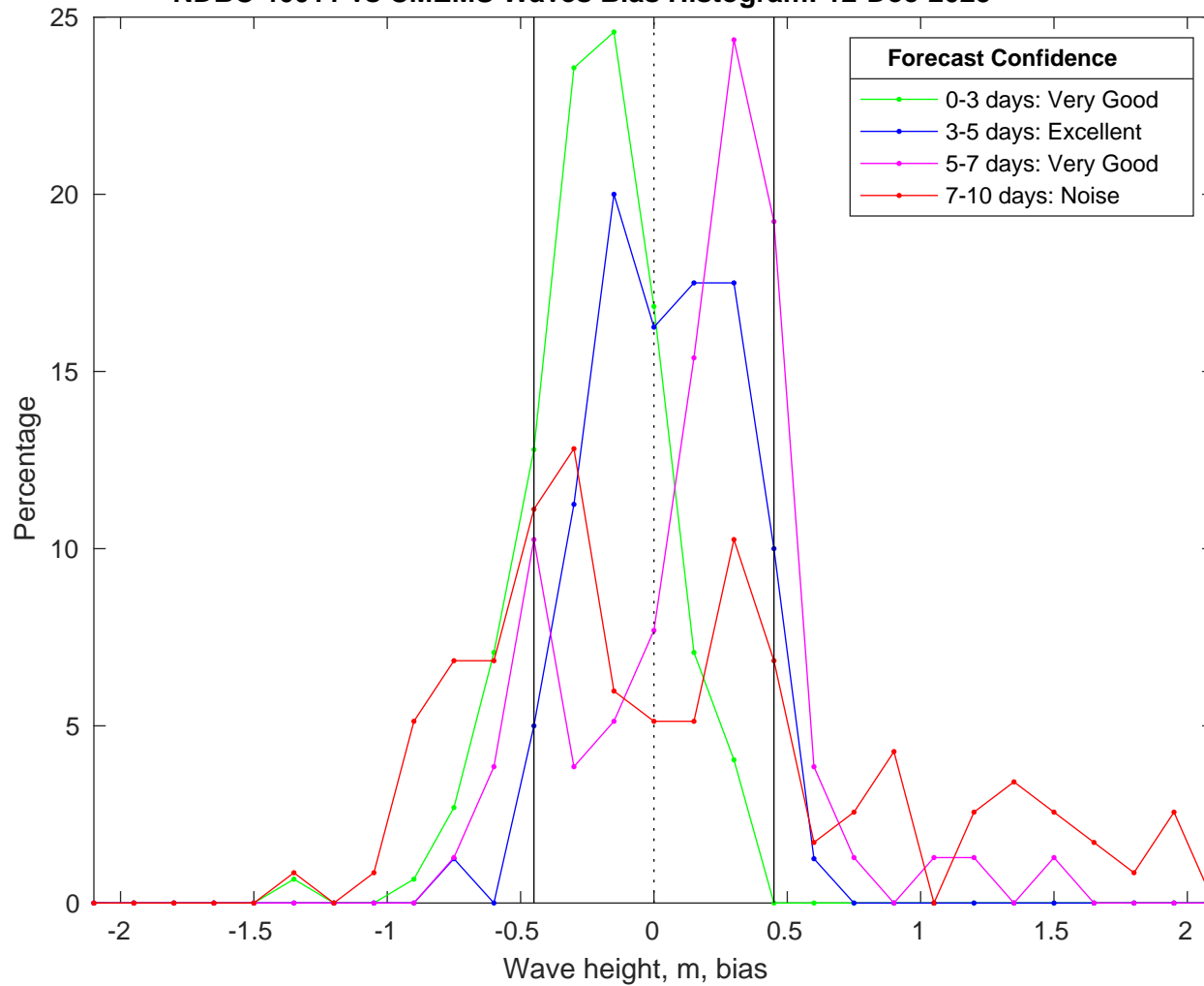
NDBC 46011 vs CMEMS Waves Bias Histogram: 12-Dec-2025
