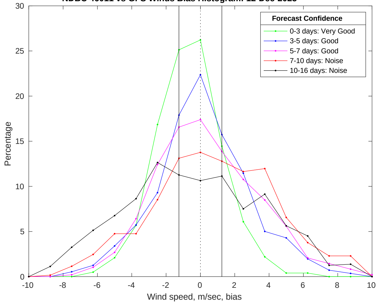
NDBC 46011 vs GFS Winds Bias Histogram: 12-Dec-2025
