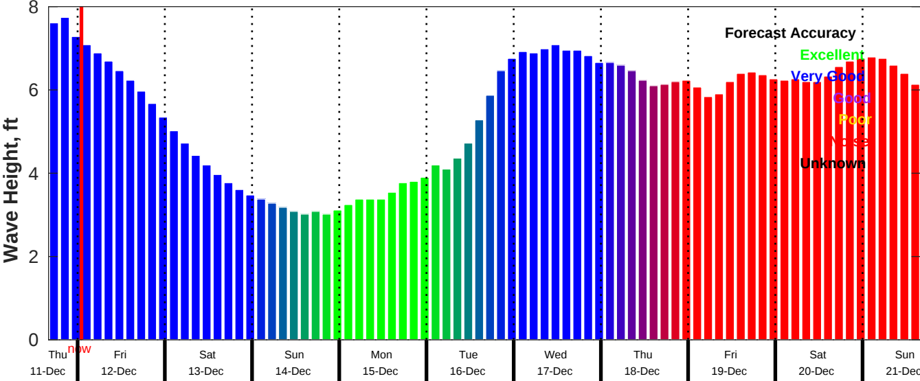
CMEMS Wave Forecast for NDBC 46011 from 11-Dec-2025 16:00:00 to 21-Dec-2025 16:00:00
