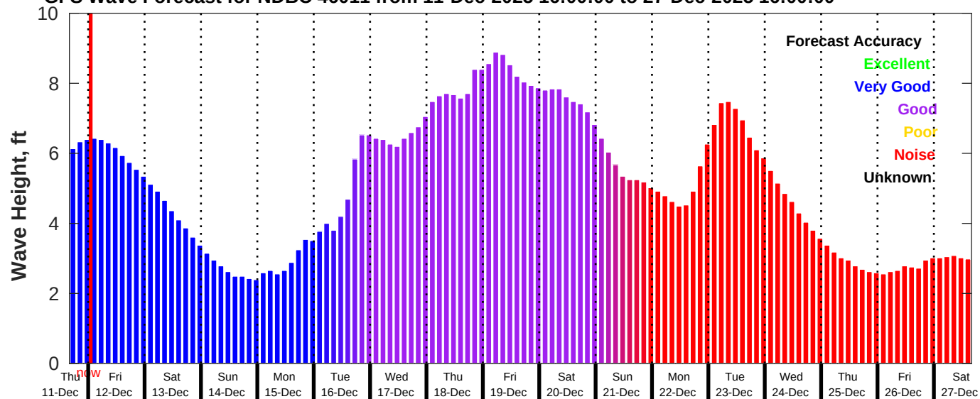
GFS Wave Forecast for NDBC 46011 from 11-Dec-2025 16:00:00 to 27-Dec-2025 16:00:00
