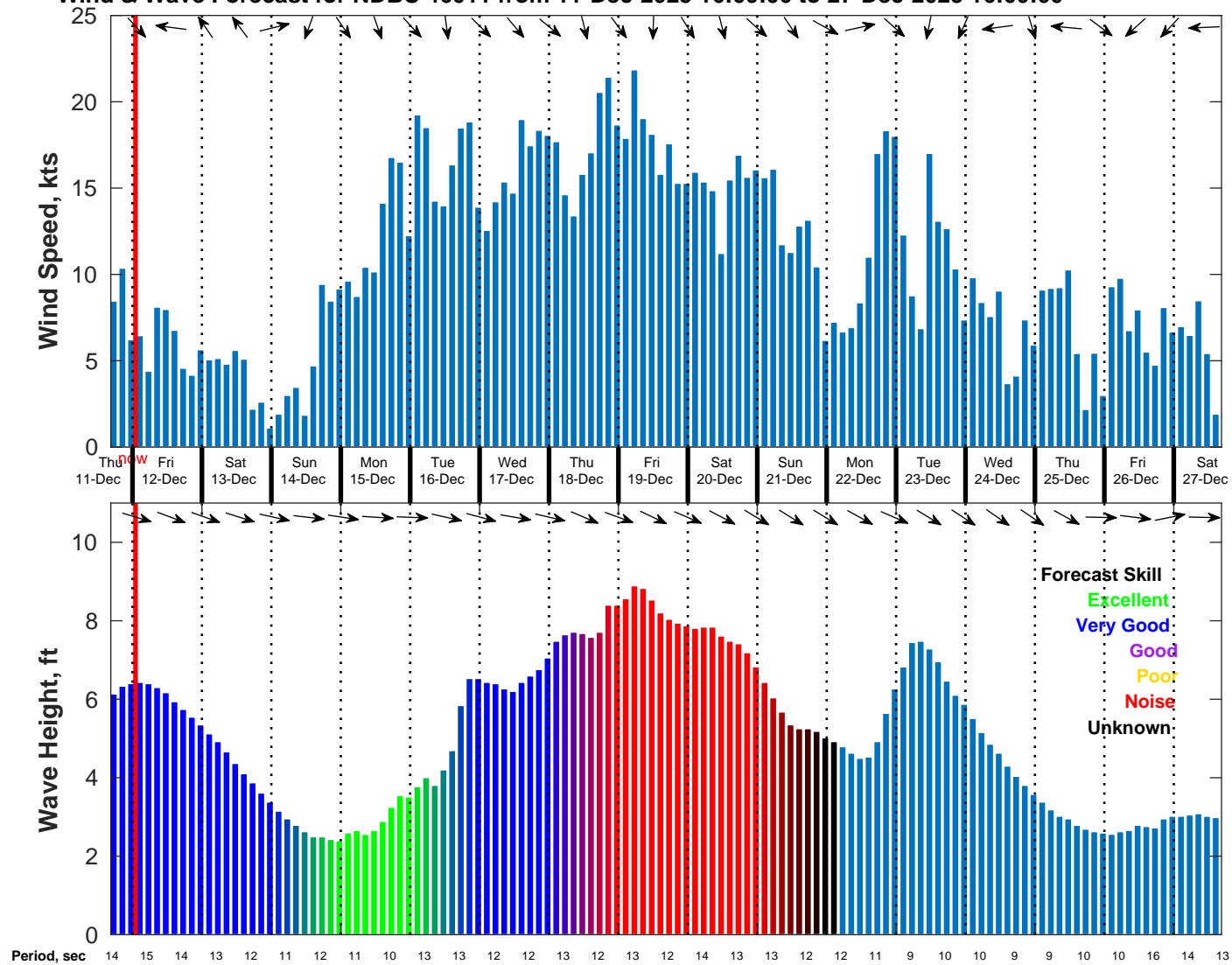
Wind & Wave Forecast for NDBC 46011 from 11-Dec-2025 16:00:00 to 27-Dec-2025 16:00:00
