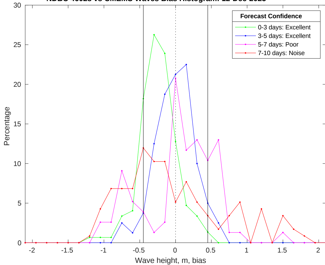
NDBC 46028 vs CMEMS Waves Bias Histogram: 12-Dec-2025
