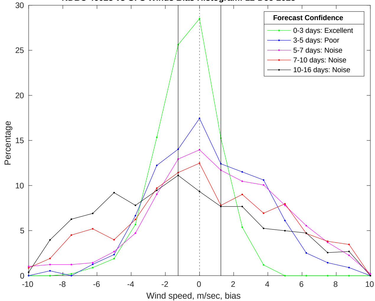
NDBC 46028 vs GFS Winds Bias Histogram: 12-Dec-2025
