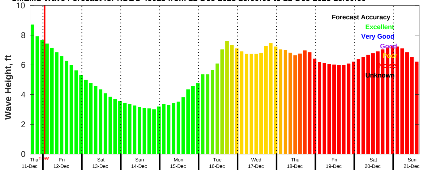
CMEMS Wave Forecast for NDBC 46028 from 11-Dec-2025 16:00:00 to 21-Dec-2025 16:00:00
