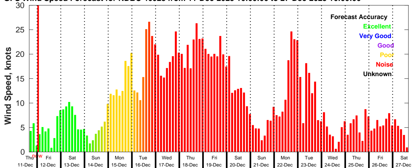
GFS Wind Speed Forecast for NDBC 46028 from 11-Dec-2025 16:00:00 to 27-Dec-2025 16:00:00
