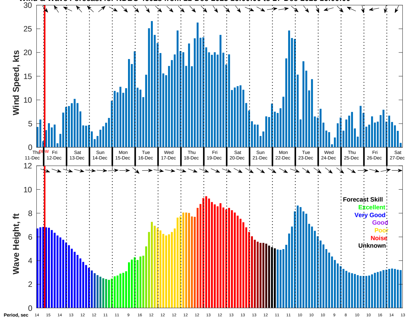
Wind & Wave Forecast for NDBC 46028 from 11-Dec-2025 16:00:00 to 27-Dec-2025 16:00:00
