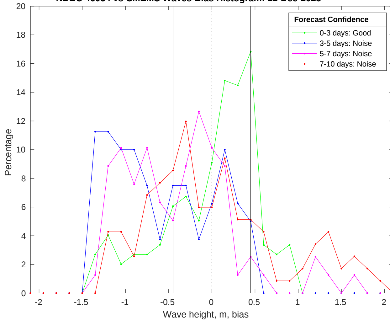
NDBC 46054 vs CMEMS Waves Bias Histogram: 12-Dec-2025
