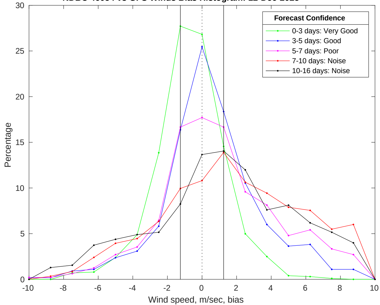
NDBC 46054 vs GFS Winds Bias Histogram: 12-Dec-2025
