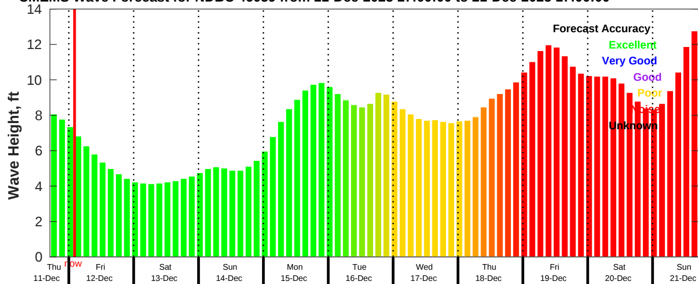
CMEMS Wave Forecast for NDBC 46059 from 11-Dec-2025 17:00:00 to 21-Dec-2025 17:00:00
