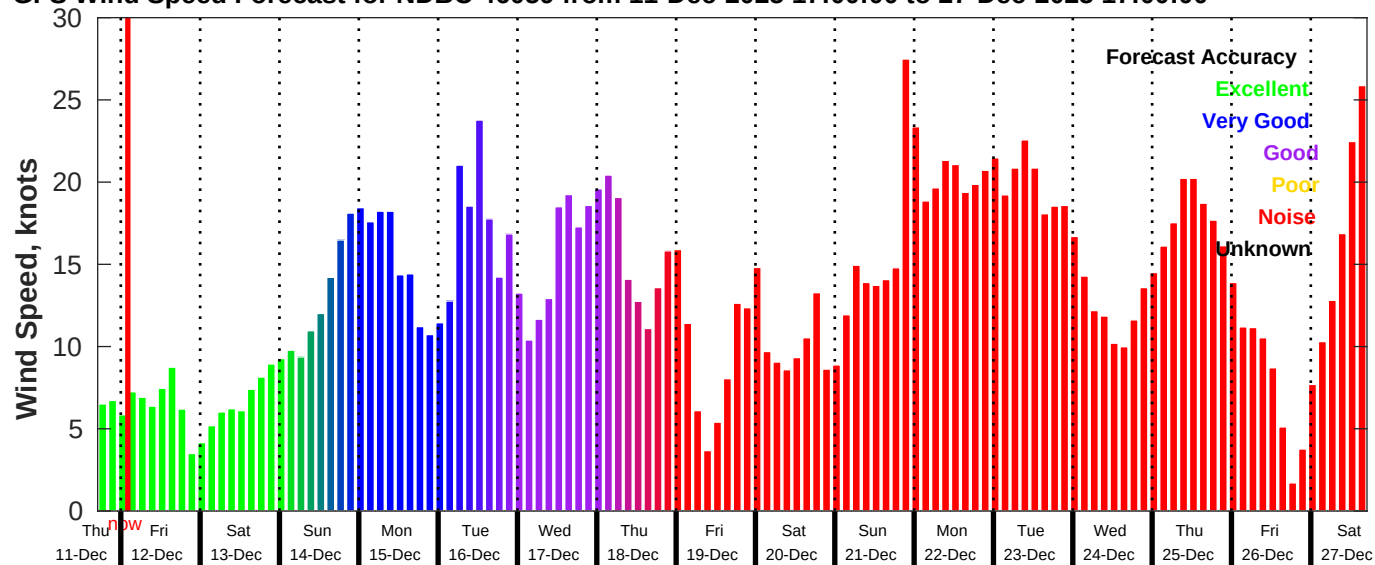
GFS Wind Speed Forecast for NDBC 46059 from 11-Dec-2025 17:00:00 to 27-Dec-2025 17:00:00
