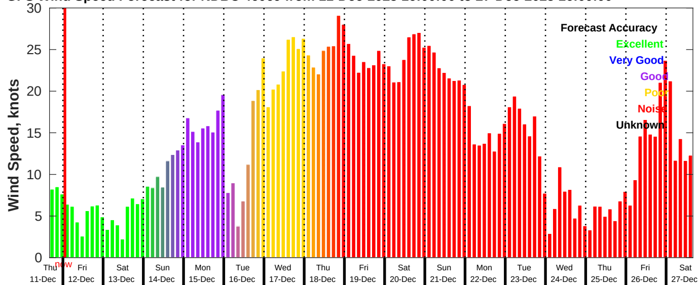
GFS Wind Speed Forecast for NDBC 46069 from 11-Dec-2025 16:00:00 to 27-Dec-2025 16:00:00
