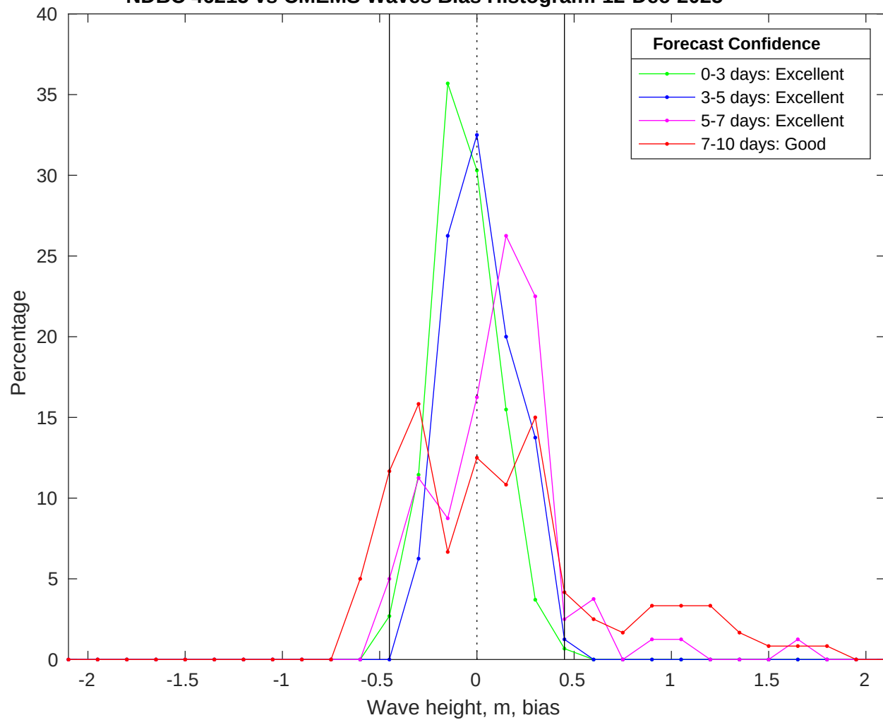
NDBC 46215 vs CMEMS Waves Bias Histogram: 12-Dec-2025
