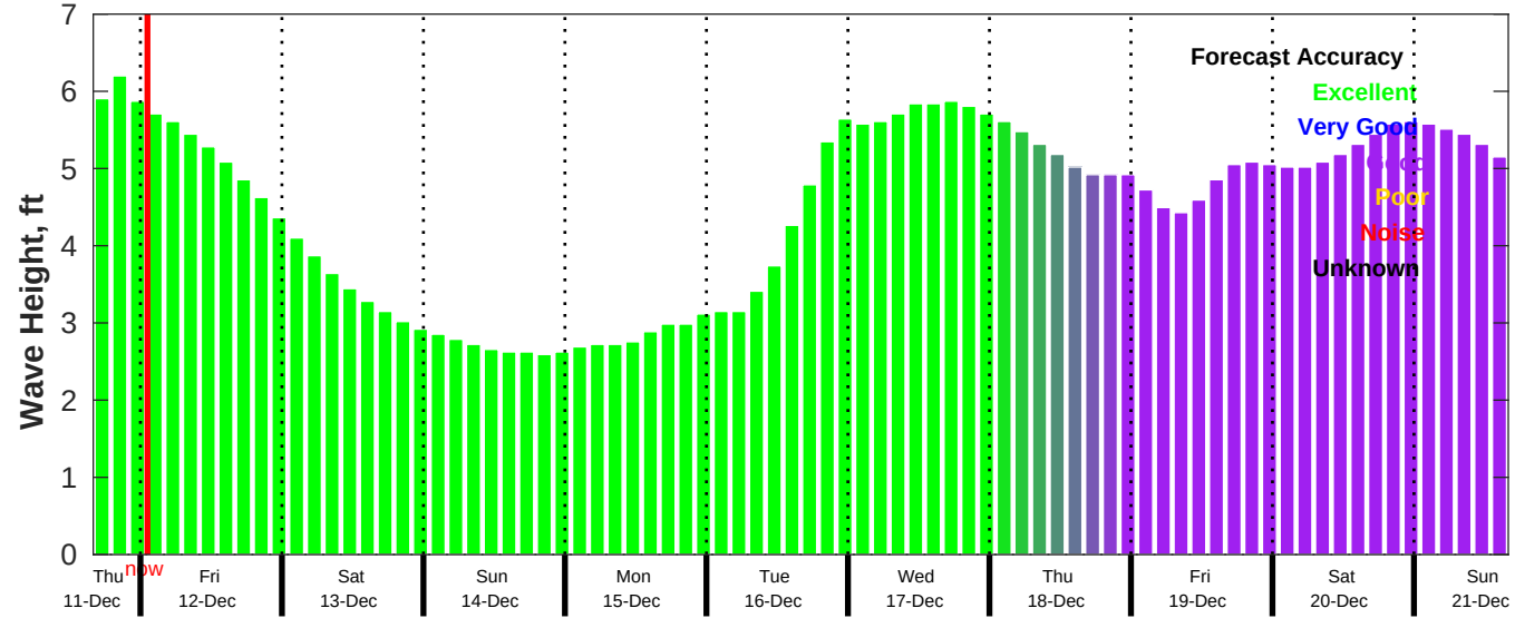
CMEMS Wave Forecast for NDBC 46215 from 11-Dec-2025 16:00:00 to 21-Dec-2025 16:00:00
